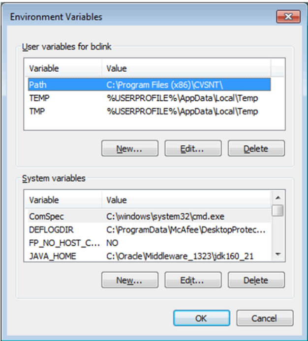
Figure 4–8 Environment Variables
